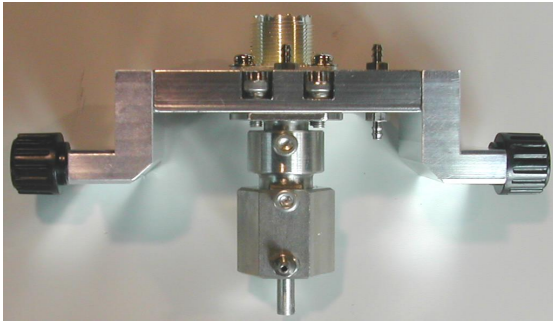
Co-axial Spinneret
