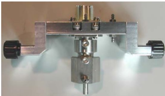
Co-axial Spinneret
