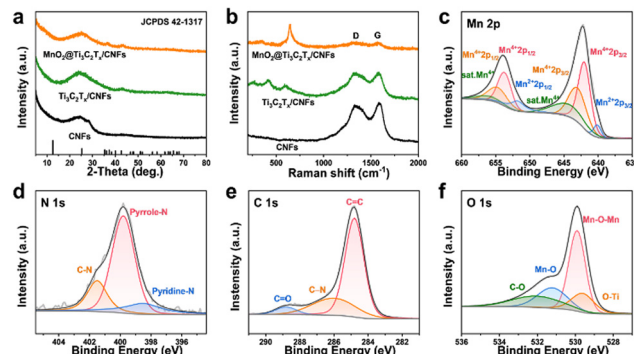
Fig. 2 (a) XRD patterns of CNFs, \text{Ti}_3\text{C}_2\text{T}_x/\text{CNFs} and \text{MnO}_2@\text{Ti}_3\text{C}_2\text{T}_x/\text{CNFs} ; (b) Raman scattering spectra of CNFs, \text{Ti}_3\text{C}_2\text{T}_x/\text{CNFs} and \text{MnO}_2@\text{Ti}_3\text{C}_2\text{T}_x/\text{CNFs} ; (c)–(f) XPS spectra of \text{MnO}_2@\text{Ti}_3\text{C}_2\text{T}_x/\text{CNFs} : (c) Mn 2p, (d) N 1s, (e) C 1s, and (f) O 1s.
