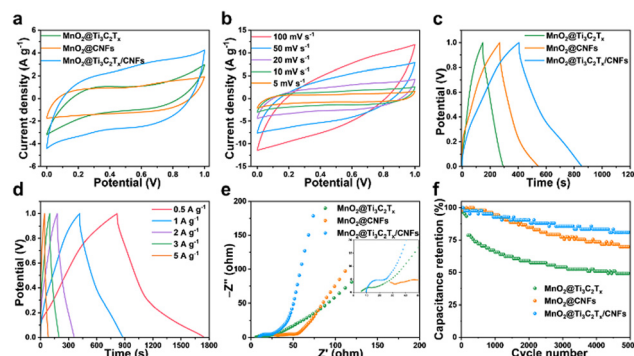
Fig. 3 The electrochemical performance of \text{MnO}_2@\text{Ti}_3\text{C}_2\text{T}_x/\text{CNFs} .
