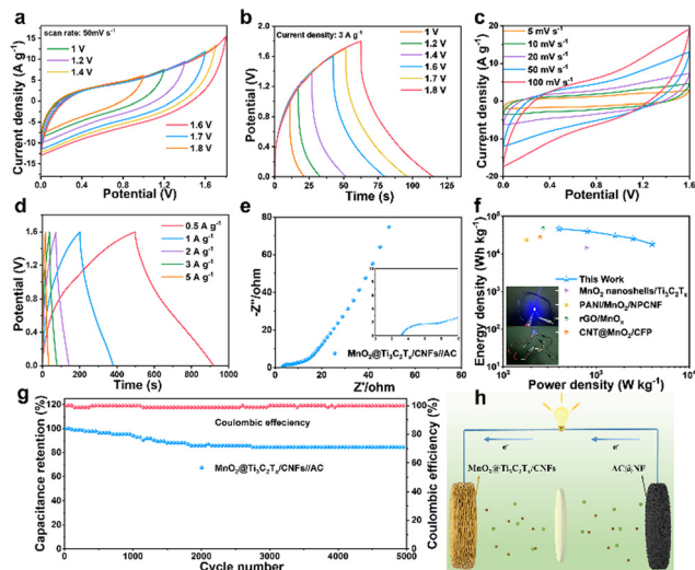
Fig. 4 The electrochemical performance of \text{MnO}_2@ \text{Ti}_3\text{C}_2\text{T}_x/\text{CNFs} // \text{AC} ASC.
