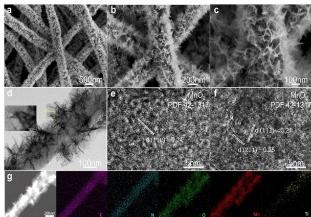
Fig. 1 (a)–(c) SEM images of the \text{MnO}_2@\text{Ti}_3\text{C}_2\text{T}_x/\text{CNFs} fibers, (d)–(f) TEM images of \text{MnO}_2@\text{Ti}_3\text{C}_2\text{T}_x/\text{CNF} fibers, and (g) EDS elemental maps of \text{MnO}_2@\text{Ti}_3\text{C}_2\text{T}_x/\text{CNFs} .
